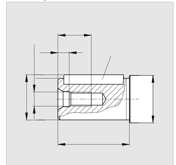
Parallel Keyed Shaft: DIN 6885
